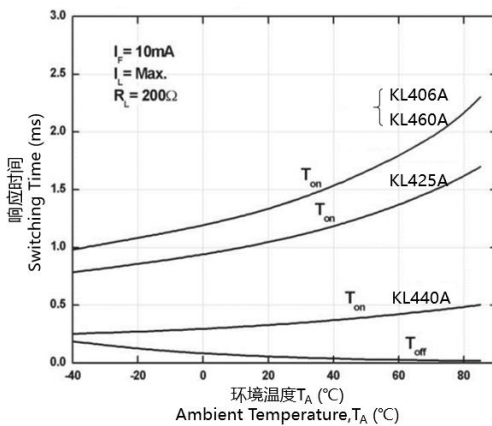
Figure 3. Switching Time vs Ambient Temperature
