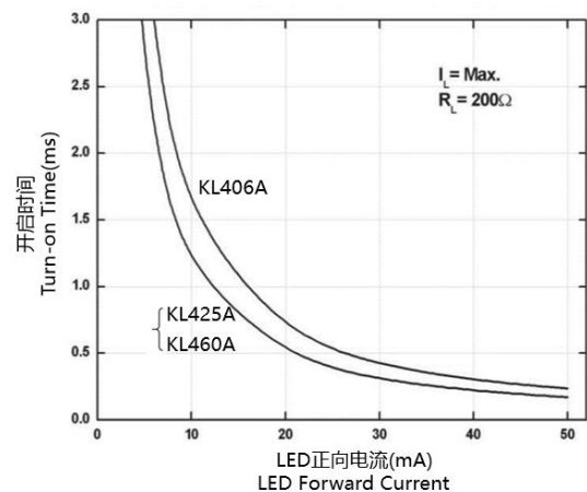
Figure 4-1. Turn-on Time vs LED Forward Current
