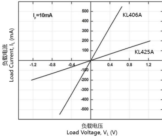
Figure 9-2. Load Current vs Load Voltage
