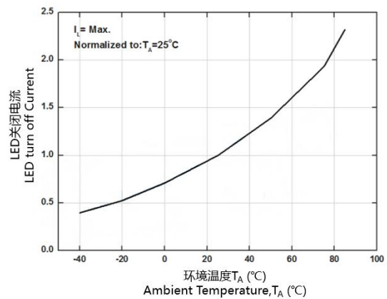
Figure 7 LED turn off Current vs Ambient Temperature
