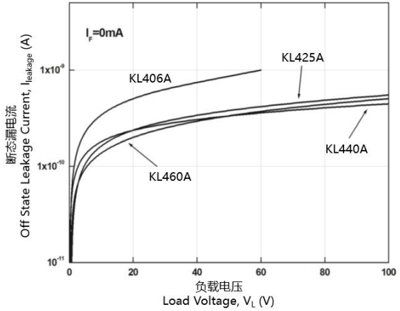
Figure 10 Off State Leakage Current vs Load Voltage
