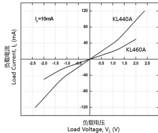
Figure 9-1 Load Current vs Load Voltage
