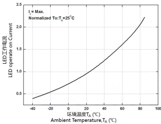
Figure 6. LED operate on Current vs Ambient Temperature
