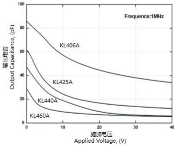
Figure 11. Output Capacitance vs Applied Voltage
