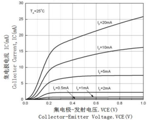
Fig.6 Collector Current vs Collector-Emission Voltage
