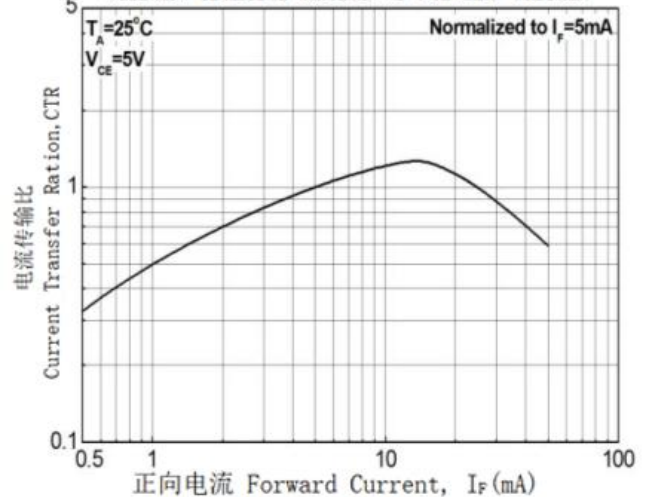
图4. 电流传输比与正向电流 Current Transfer Ratio vs Forward Current
