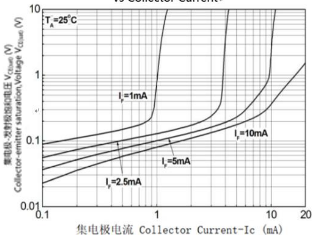
图5 集电极-发射极饱和电压与集电极电流 Figure 5. Collector-Emitter Saturation Voltage vs Collector Current.
