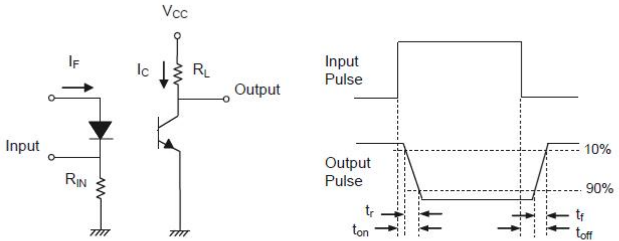
Fig7. Switching Time Test Circuit & Waveforms
